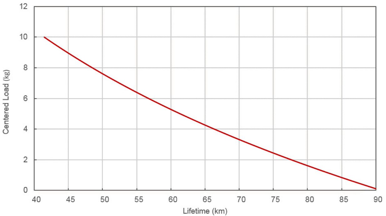
LSM Linear Bearing Lifetime
